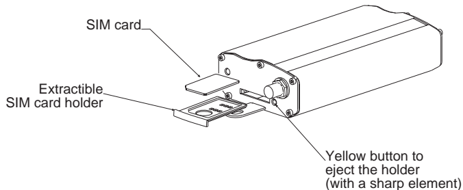
Figure 5 SIM card holder
