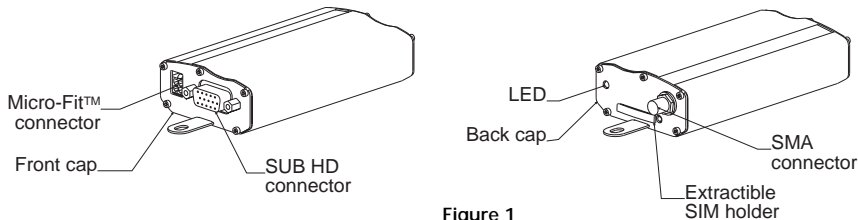
Figure 1 Modem presentation
